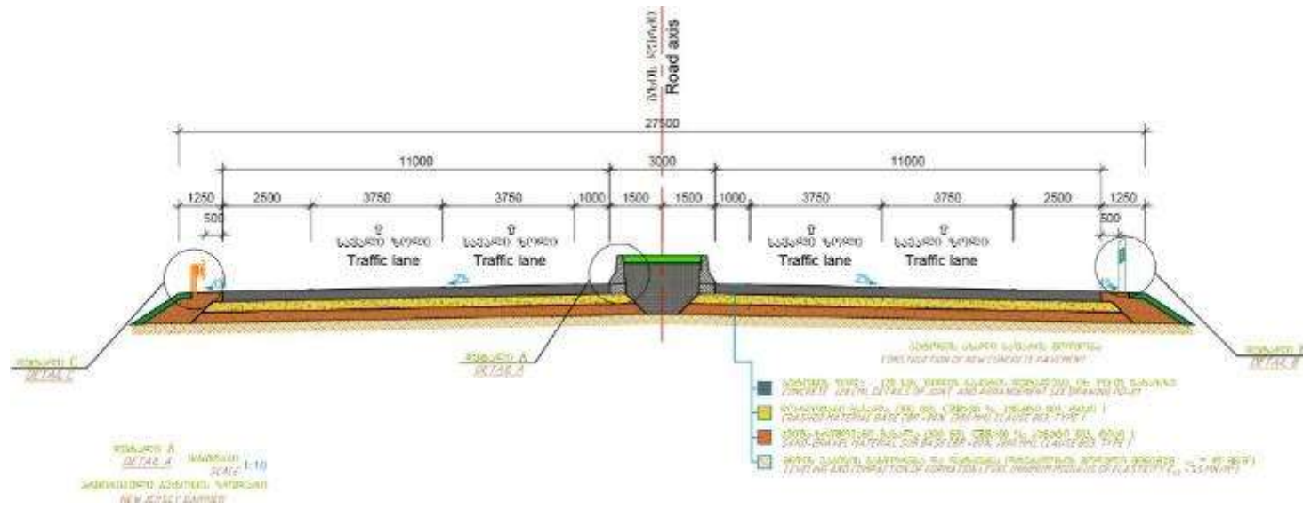
Figure 4.3.1. Typical cross sections of the new road
