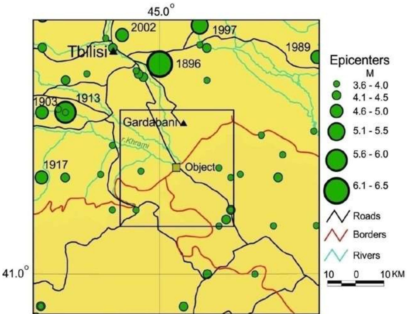
Figure 5.2.3.4.1. Map of moderate and strong earthquakes epicenters ( M > 3.5 ).
